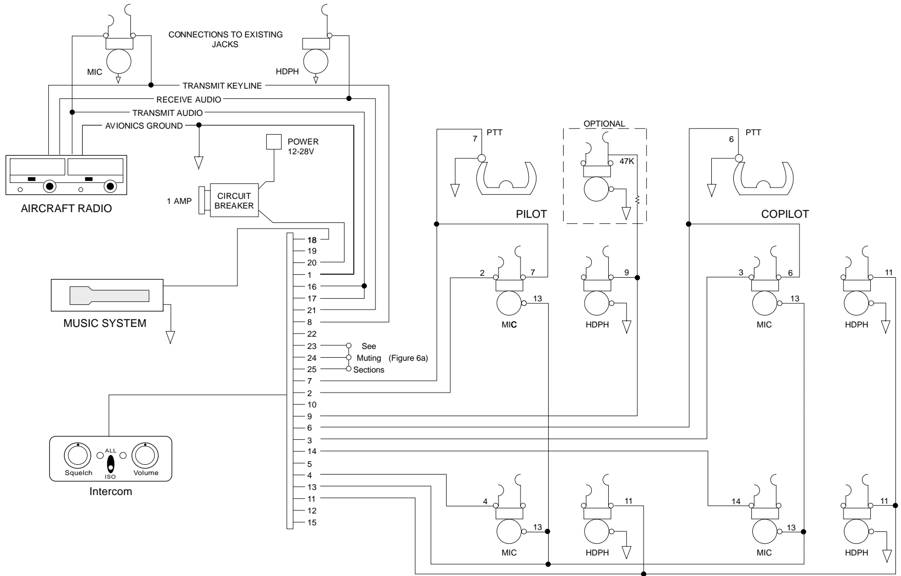
Fig. 12 Connection Schematic
